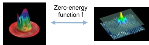
Quantum state of x
