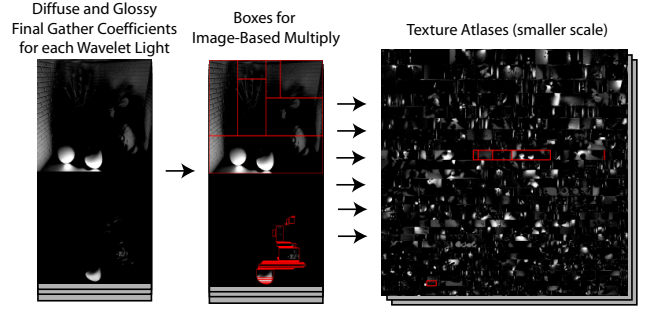
Figure 4: Data layout used to efficiently encode the sparse image-based multiplication.
