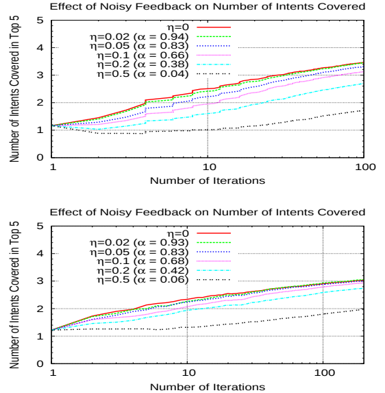
Figure 3: Effect of \eta on performance of the algorithm for users that are purely seeking diversity (number in bracket indicates the effective \alpha of the feedback); top: RCV-1, bottom: 20NG.
