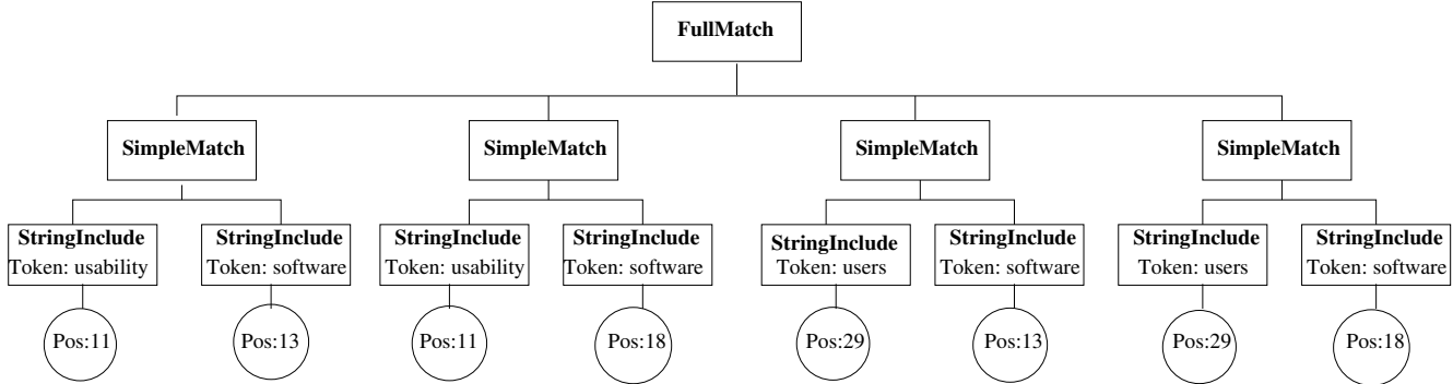
Figure 3: FullMatch for 'usability' with stems
